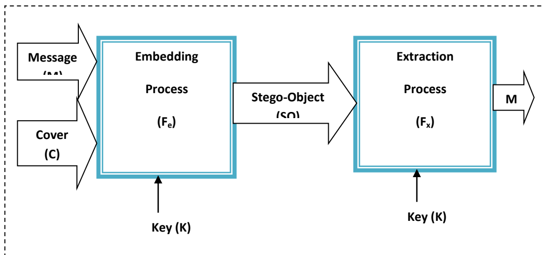
Figure 2 Basic model of steganography
