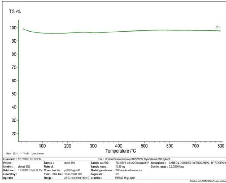
Figure A1. TGA analysis graph for sample 5
