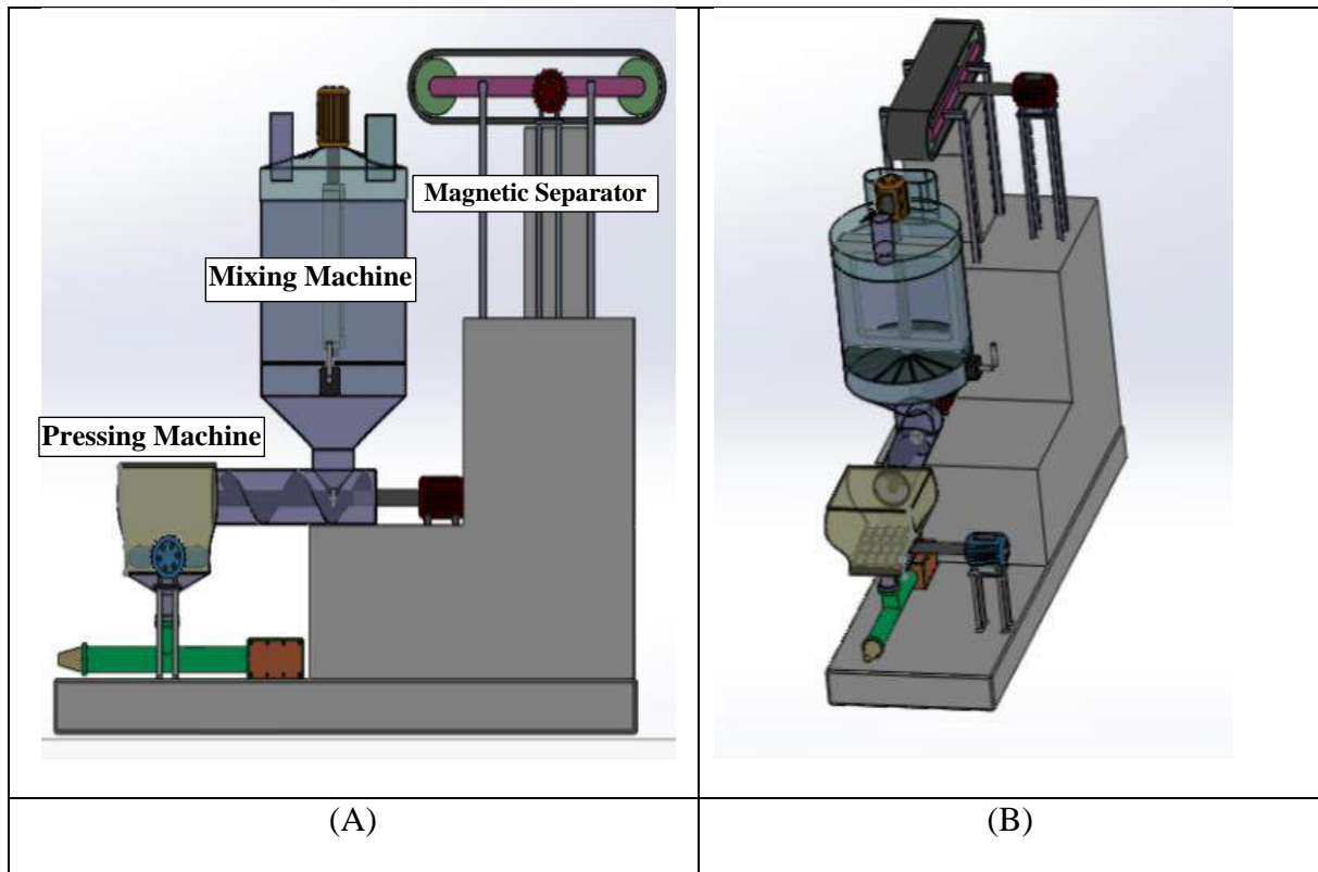
Figure 11. A and B are industrial briquette carbon fuel pressing machines.
