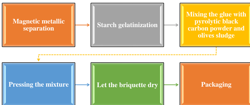
Figure 13. Summary of manufactured process for the industrial briquette carbon fuel.
