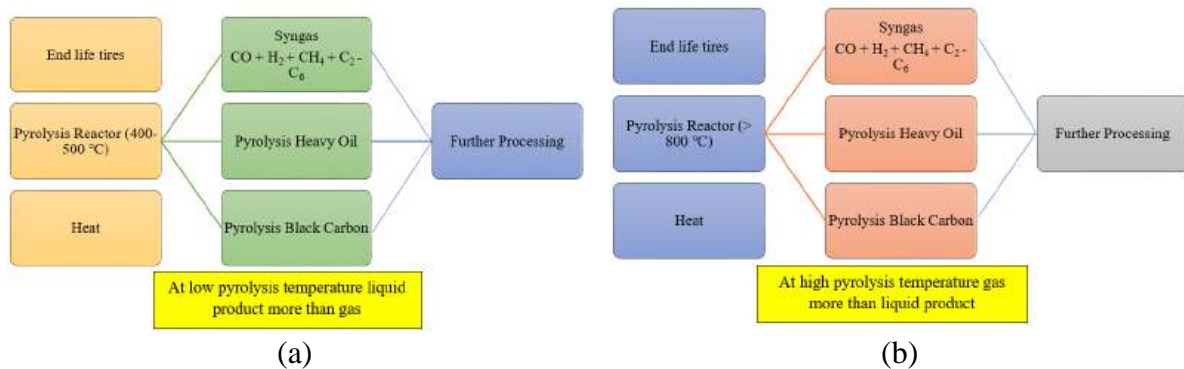
Figure 2. Schematic presentation of a (a) low and (b) high pyrolysis temperature (Hoang et al. 2020).
