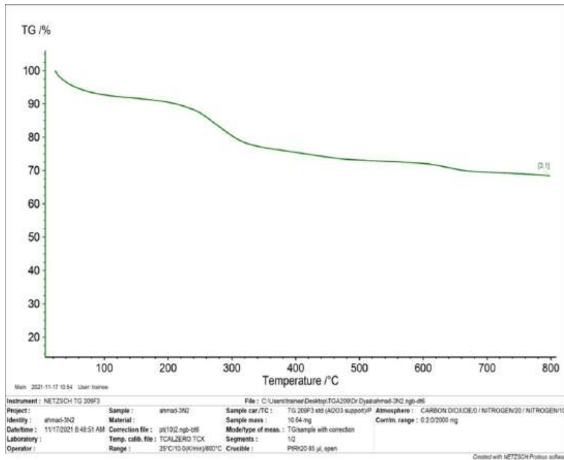
Figure A2. TGA Analysis Graph for Sample 3.
