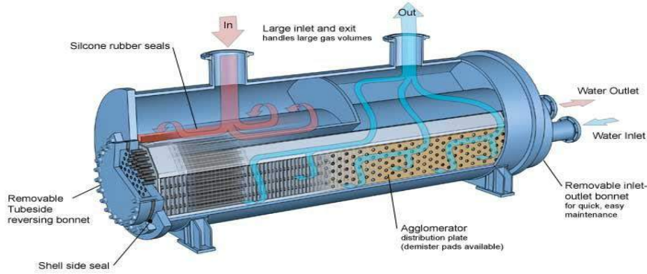
Figure 8 shell and tube heat exchanger
