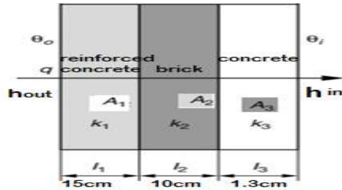
Figure 13 The composite wall
